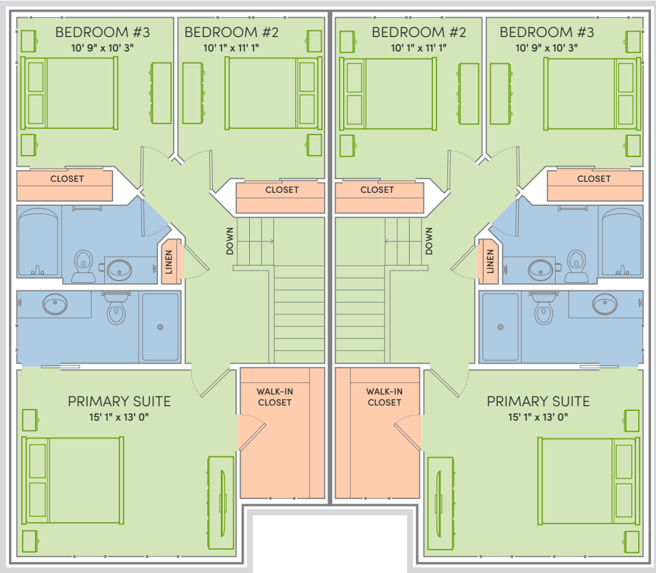
THE ALDO UNIT A: SECOND FLOOR
