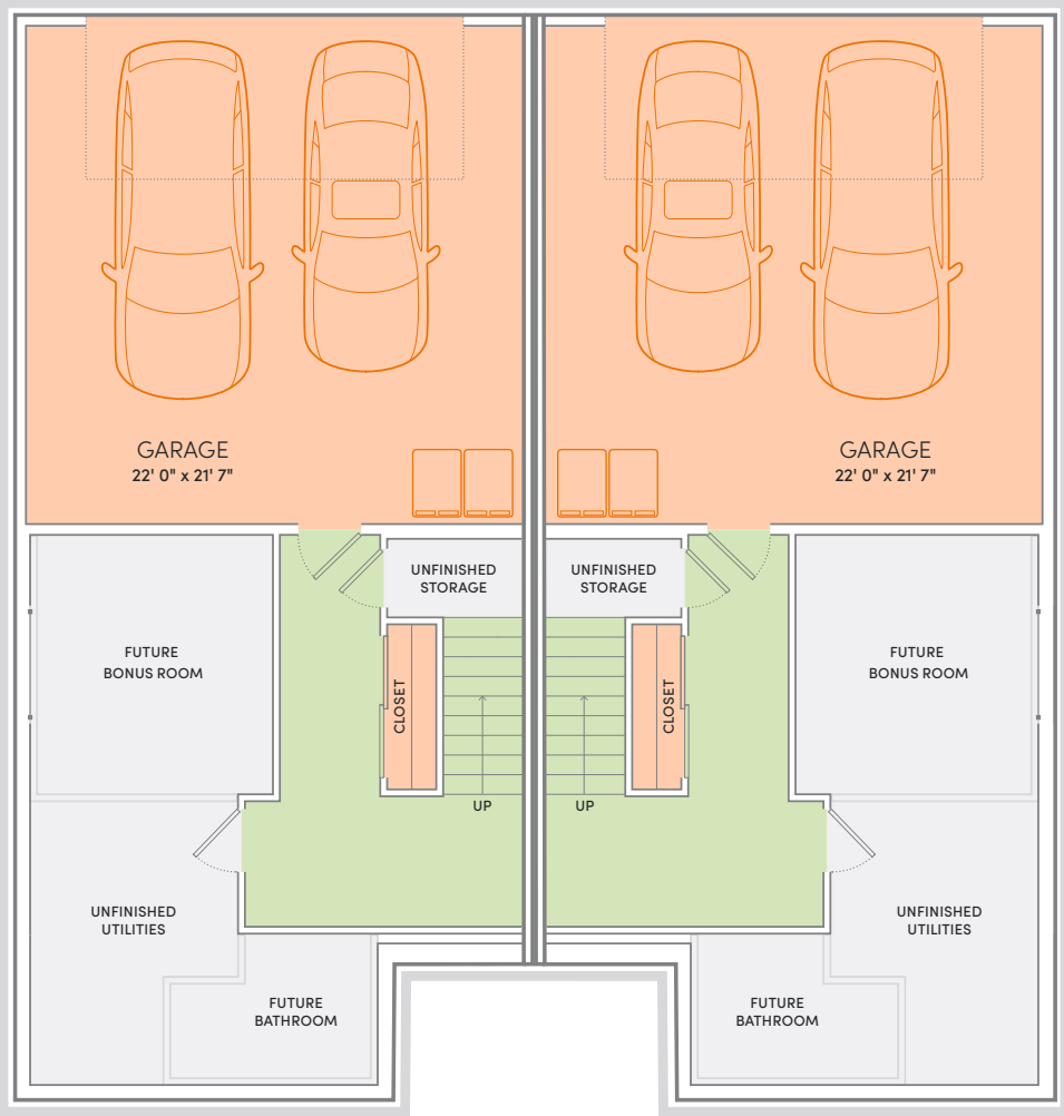
THE ALDO UNIT A: LOWER LEVEL
