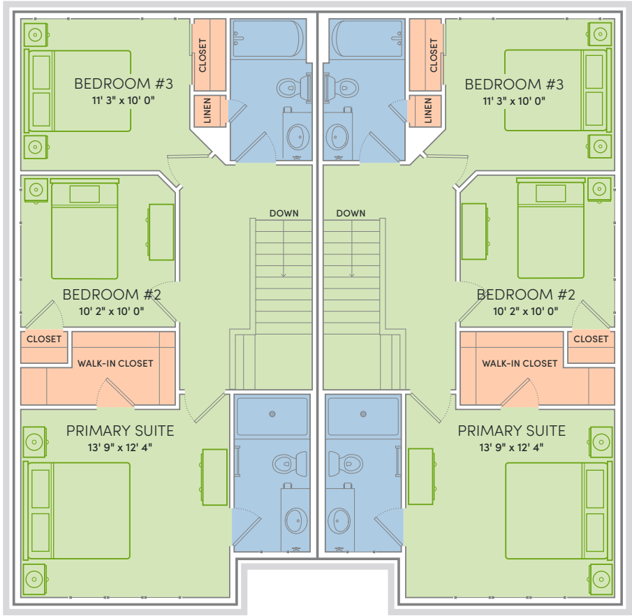
THE TRIBECA UNIT A: SECOND FLOOR
