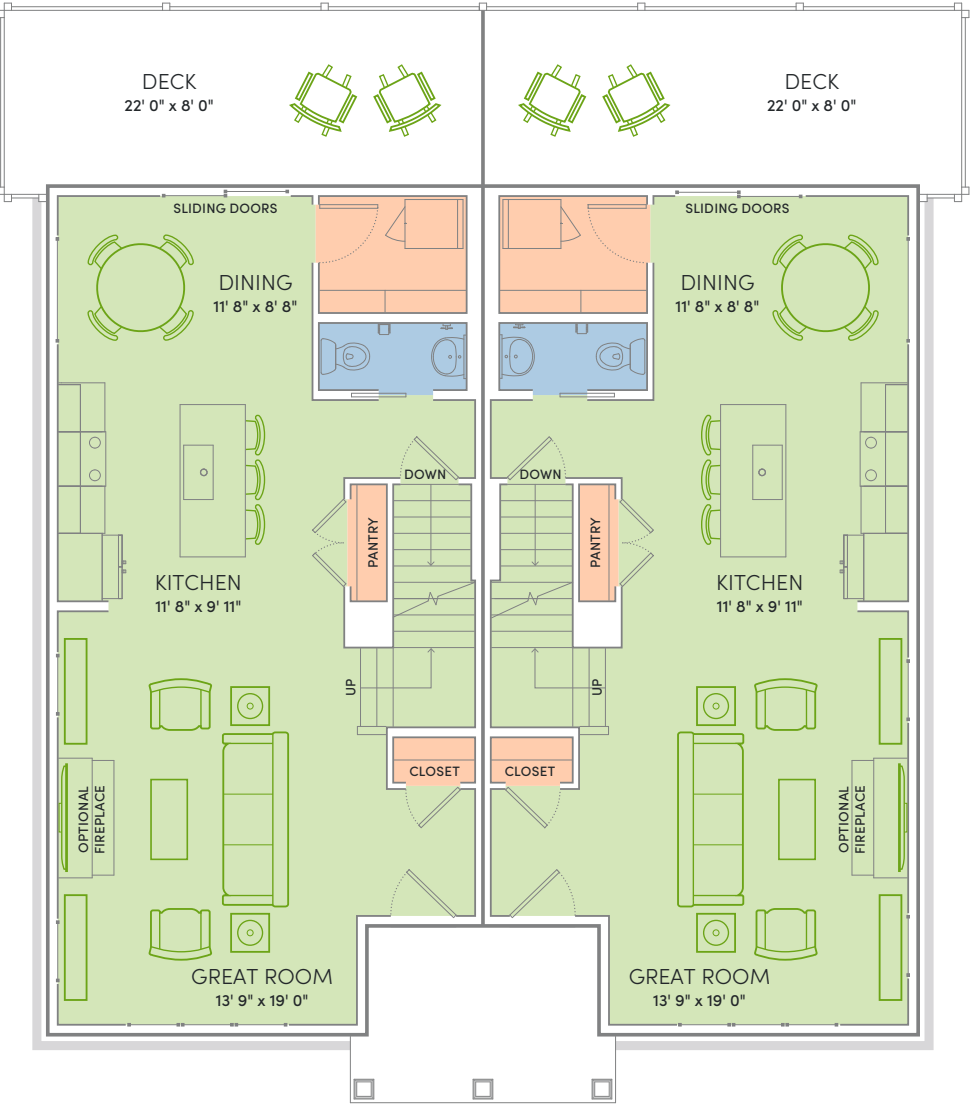
THE TRIBECA UNIT A: FIRST FLOOR
